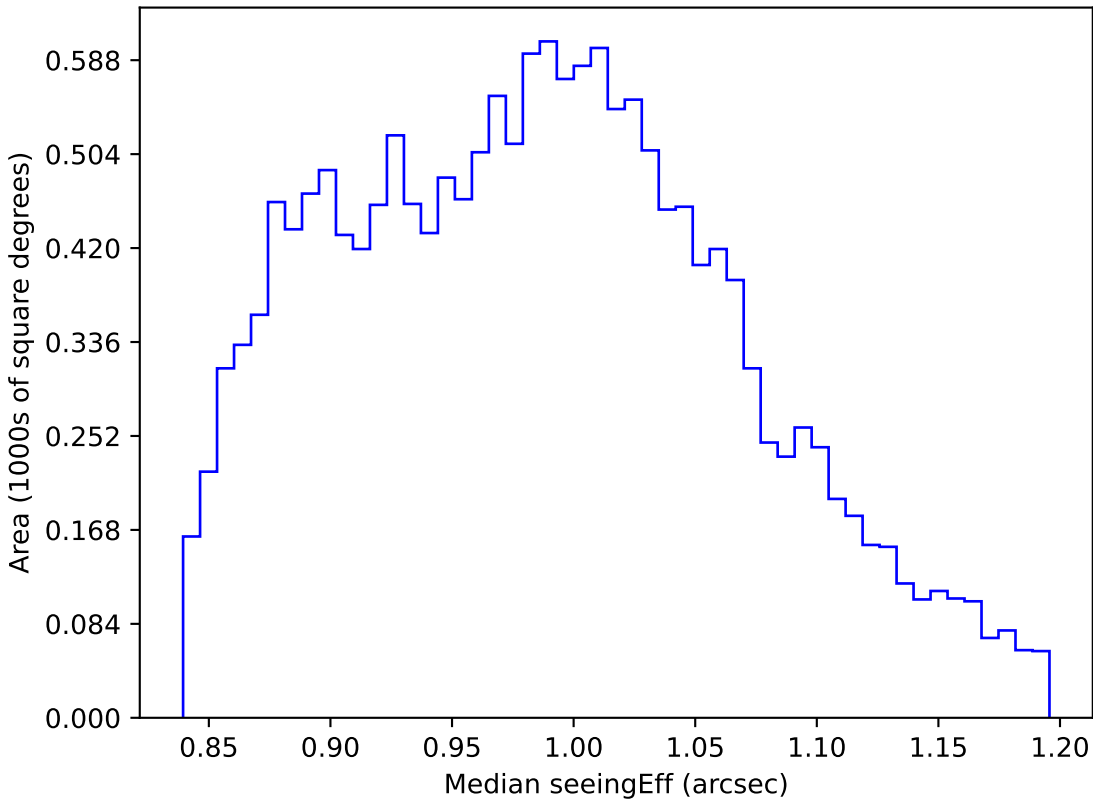
scp_reweight_v3.3_10yrs WFD i band: Median seeingEff
