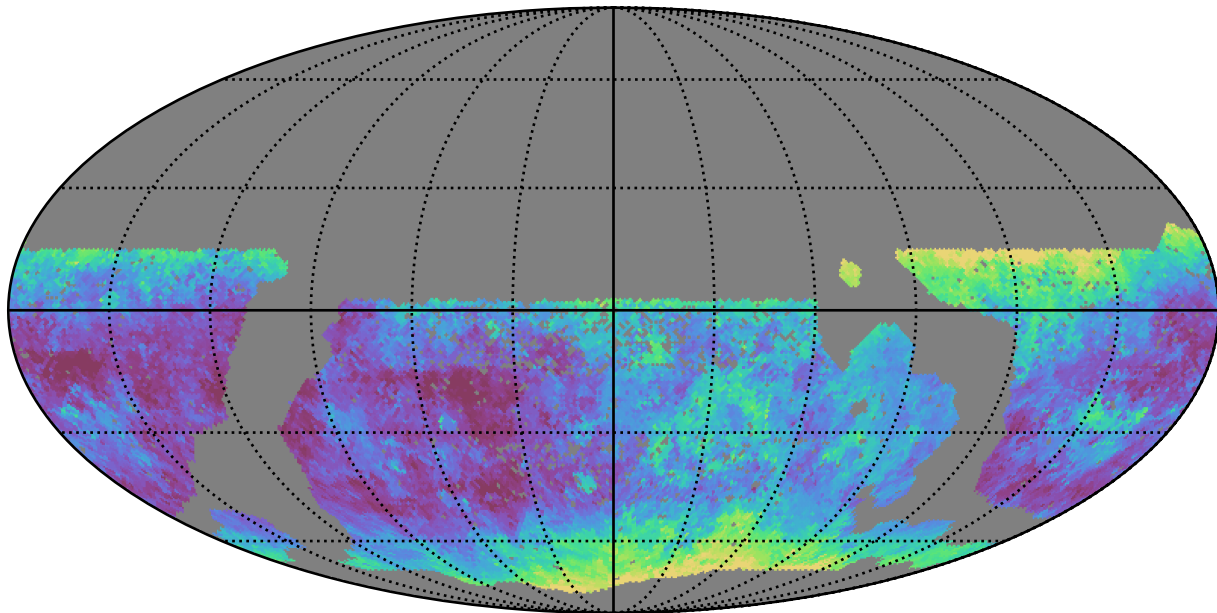
scp_reweight_v3.3_10yrs WFD g band: Median seeingEff
