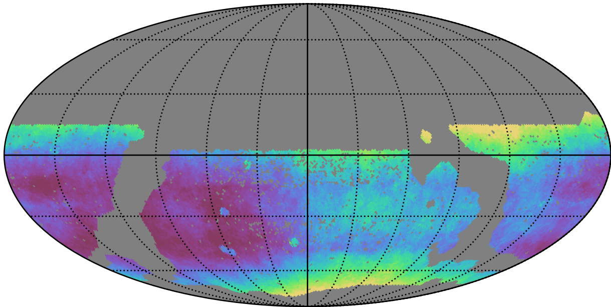
scp_reweight_v3.3_10yrs WFD all bands: Median seeingEff
