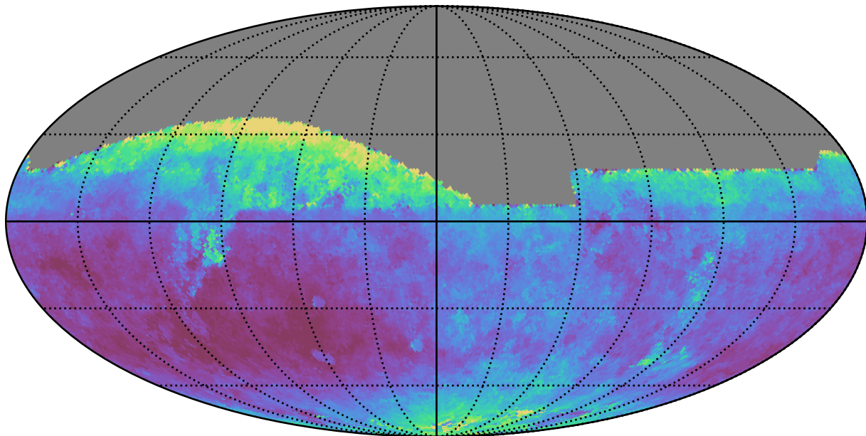
scp_reweight_v3.3_10yrs All sky z band: Median seeingEff
