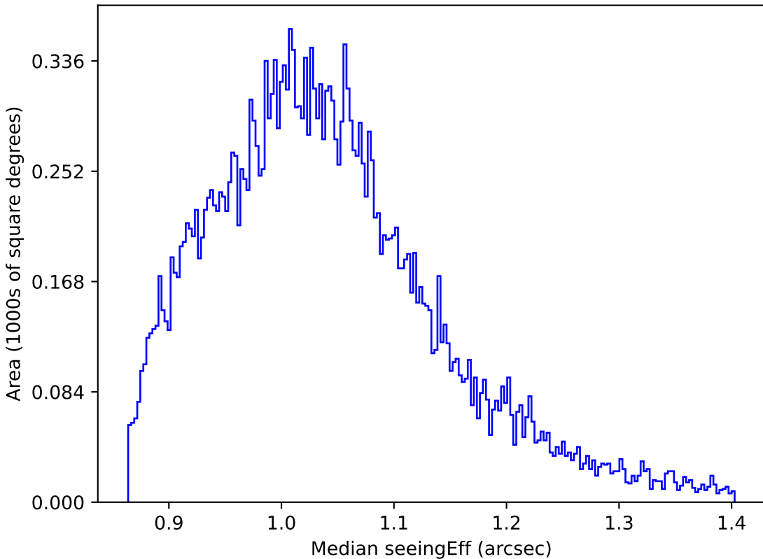
scp_reweight_v3.3_10yrs All sky z band: Median seeingEff
