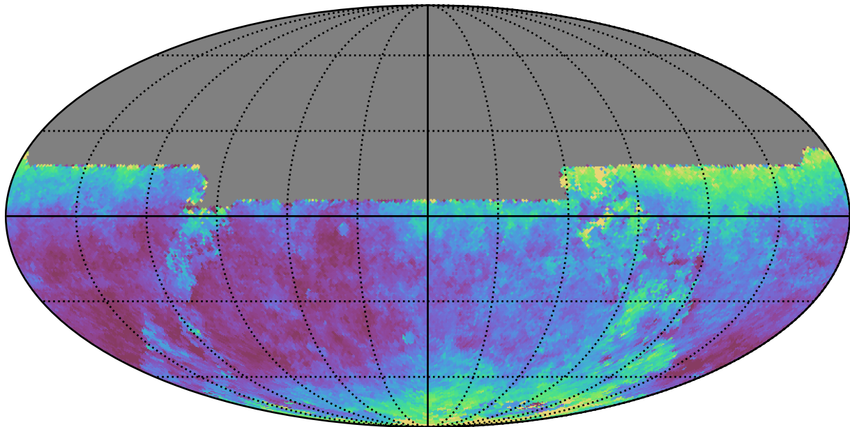
scp_reweight_v3.3_10yrs All sky y band: Median seeingEff
