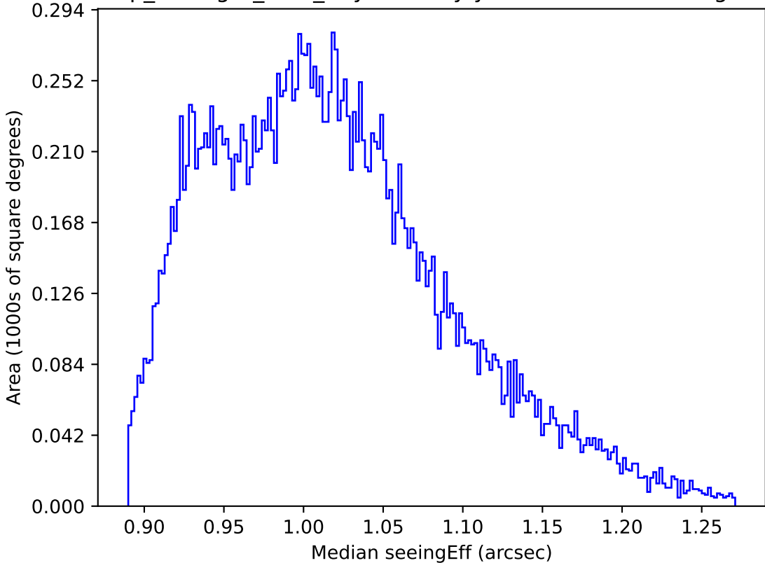
scp_reweight_v3.3_10yrs All sky y band: Median seeingEff
