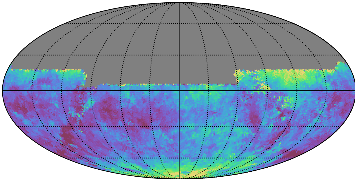
scp_reweight_v3.3_10yrs All sky u band: Median seeingEff
