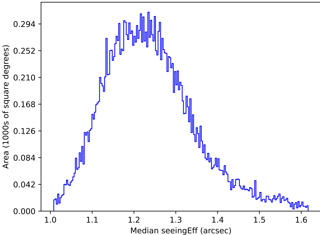
scp_reweight_v3.3_10yrs All sky u band: Median seeingEff
