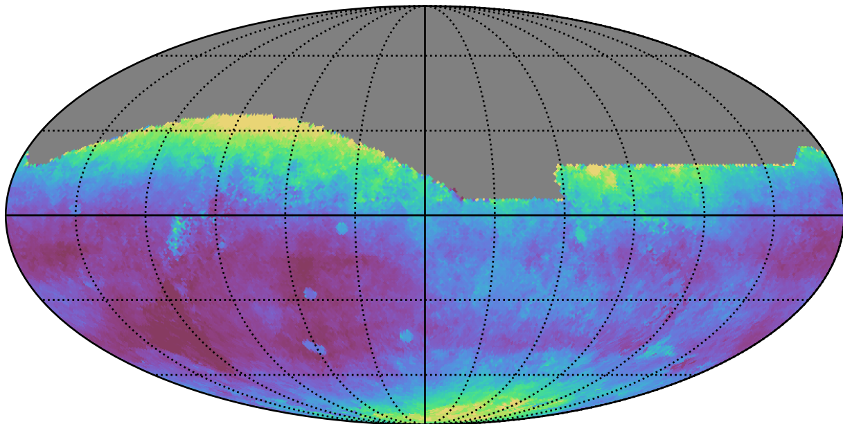
scp_reweight_v3.3_10yrs All sky r band: Median seeingEff
