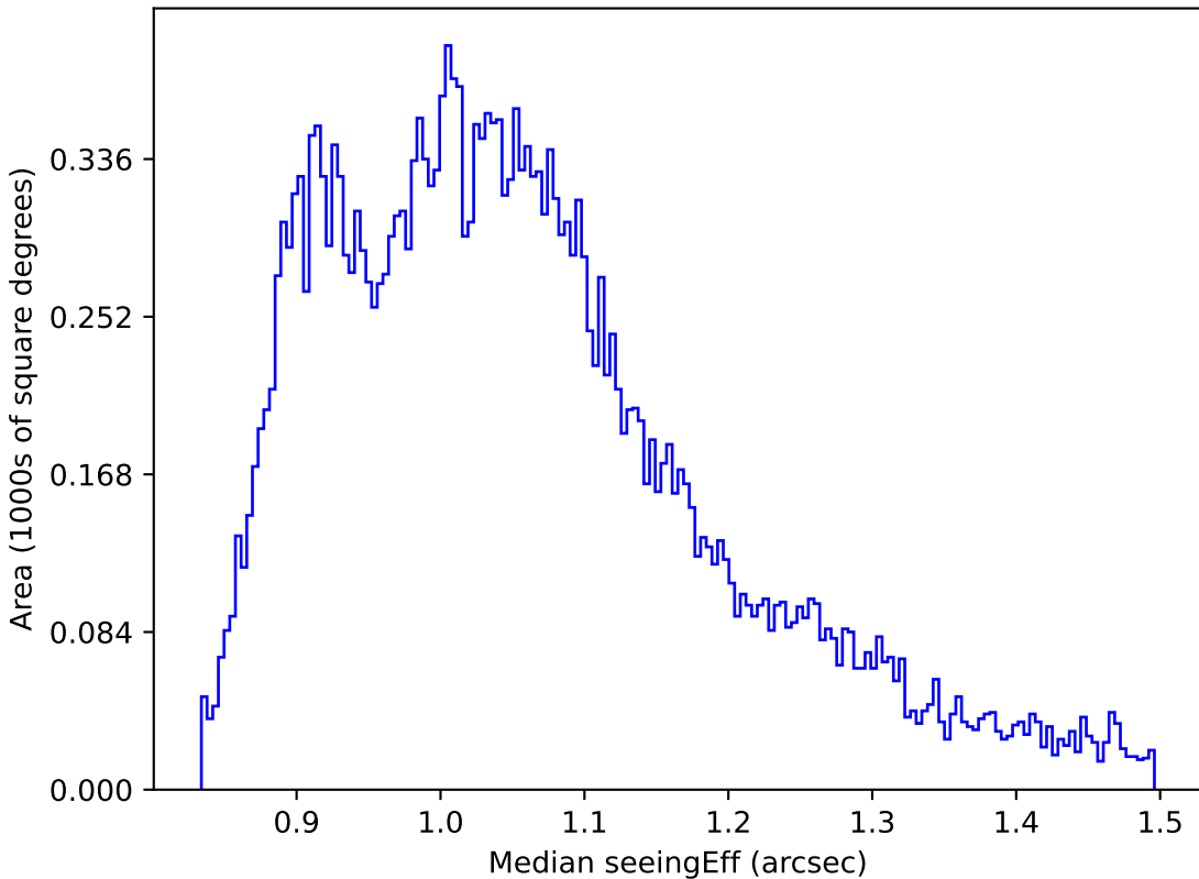
scp_reweight_v3.3_10yrs All sky r band: Median seeingEff
