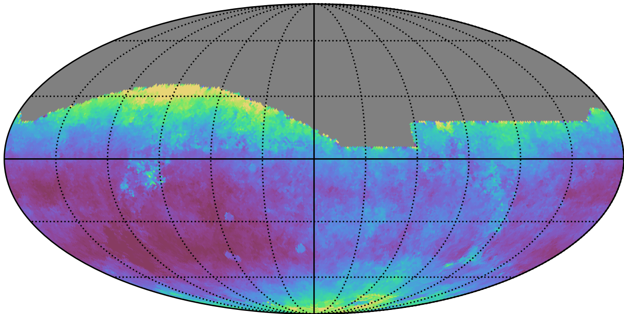
scp_reweight_v3.3_10yrs All sky i band: Median seeingEff
