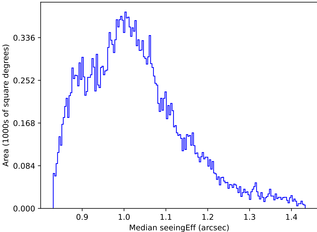
scp_reweight_v3.3_10yrs All sky i band: Median seeingEff
