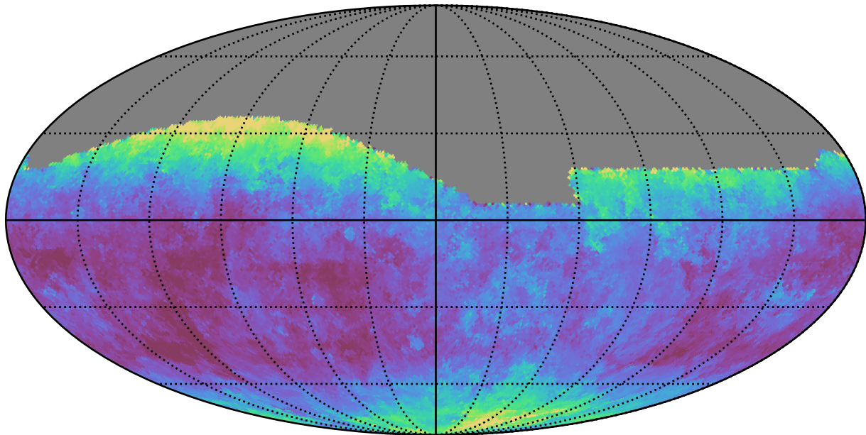
scp_reweight_v3.3_10yrs All sky g band: Median seeingEff
