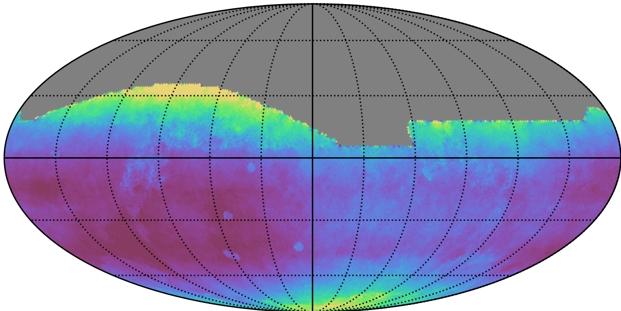
scp_reweight_v3.3_10yrs All sky all bands: Median seeingEff
