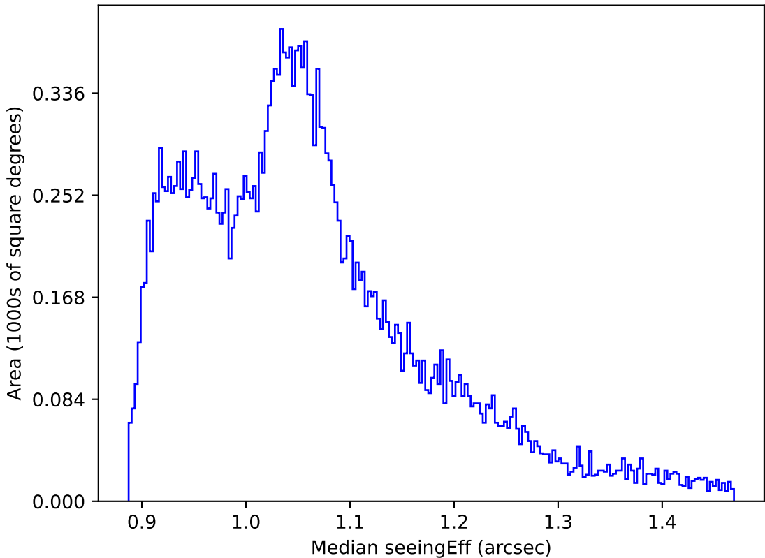
scp_reweight_v3.3_10yrs All sky all bands: Median seeingEff
