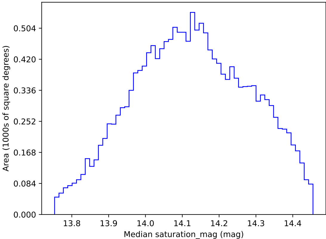
scp_reweight_v3.3_10yrs WFD z band: Median saturation_mag
