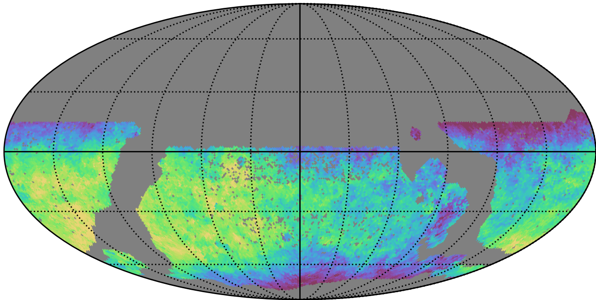
scp_reweight_v3.3_10yrs WFD y band: Median saturation_mag
