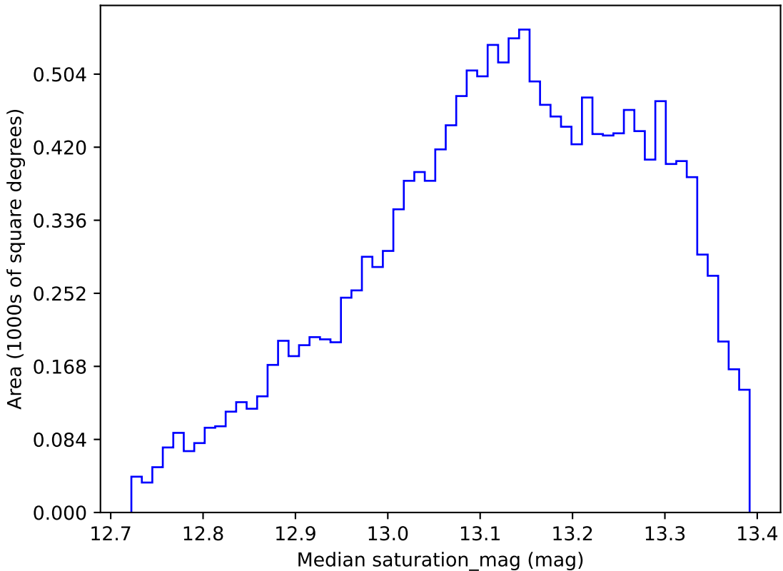
scp_reweight_v3.3_10yrs WFD y band: Median saturation_mag
