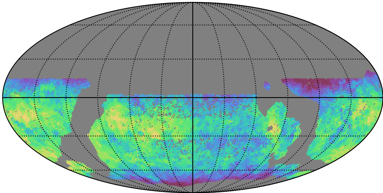
scp_reweight_v3.3_10yrs WFD u band: Median saturation_mag
