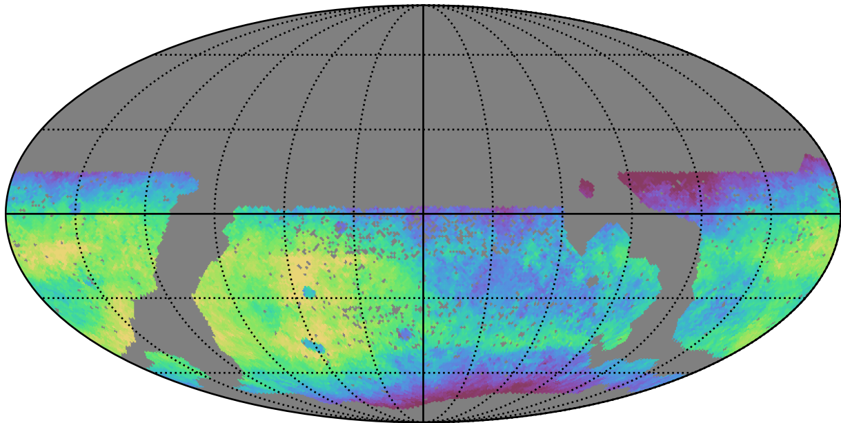
scp_reweight_v3.3_10yrs WFD r band: Median saturation_mag
