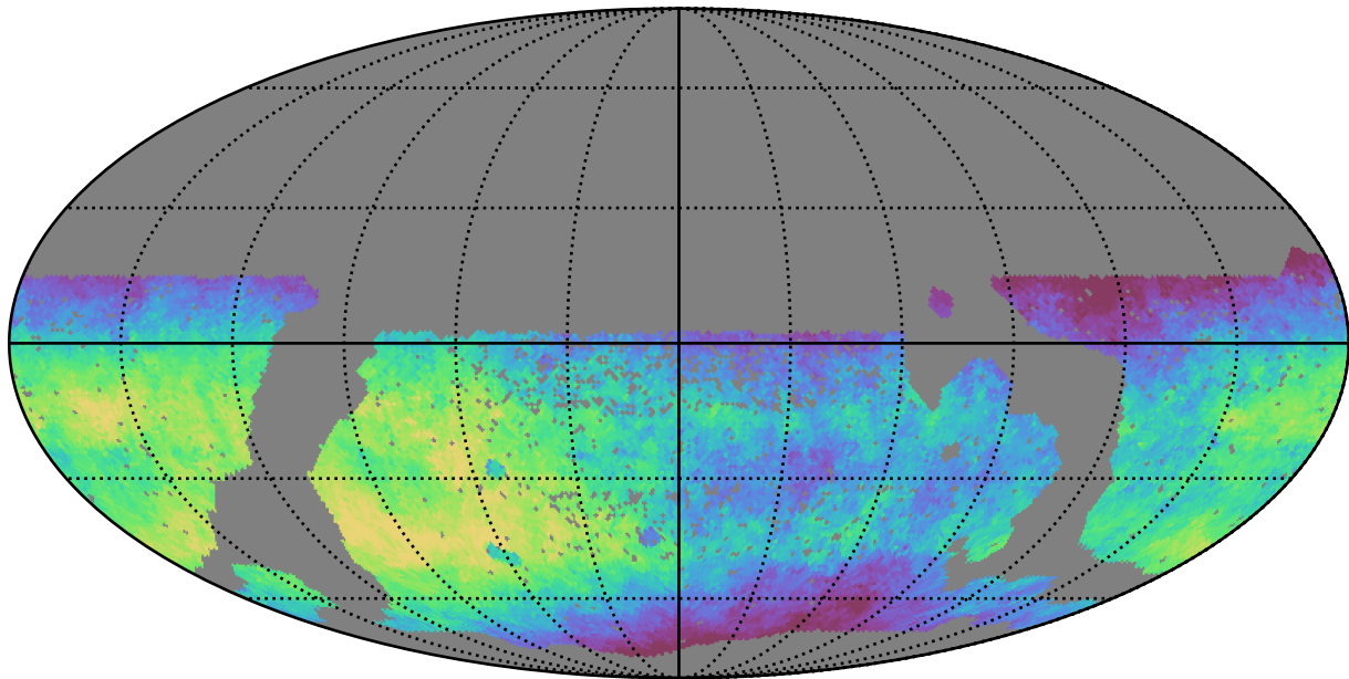
scp_reweight_v3.3_10yrs WFD i band: Median saturation_mag
