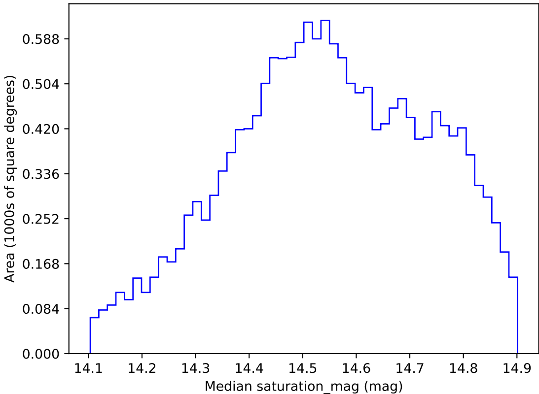
scp_reweight_v3.3_10yrs WFD i band: Median saturation_mag
