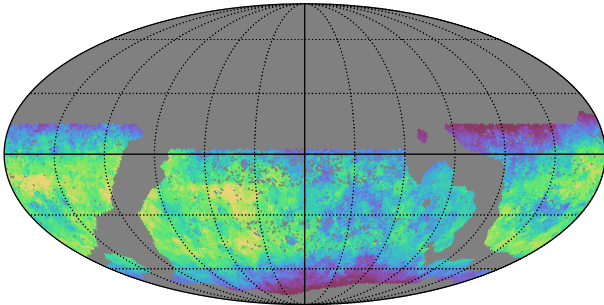
scp_reweight_v3.3_10yrs WFD g band: Median saturation_mag
