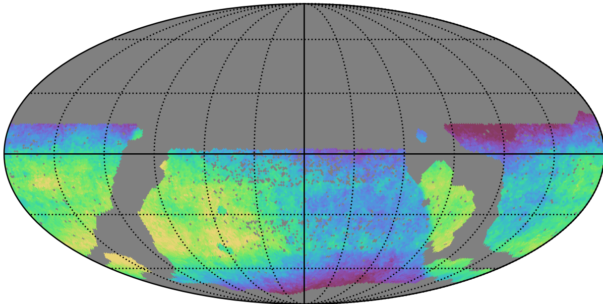
scp_reweight_v3.3_10yrs WFD all bands: Median saturation_mag
