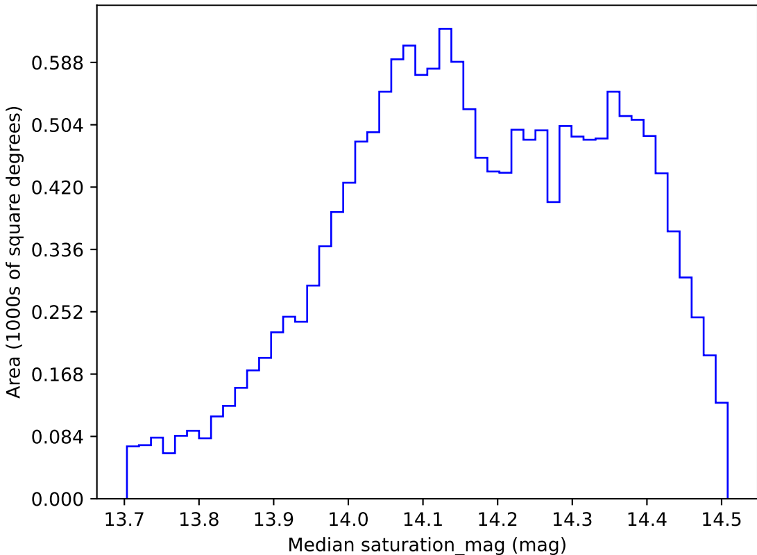
scp_reweight_v3.3_10yrs WFD all bands: Median saturation_mag
