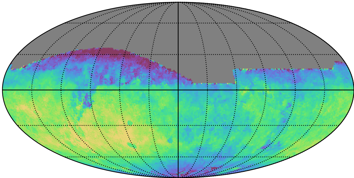
scp_reweight_v3.3_10yrs All sky z band: Median saturation_mag
