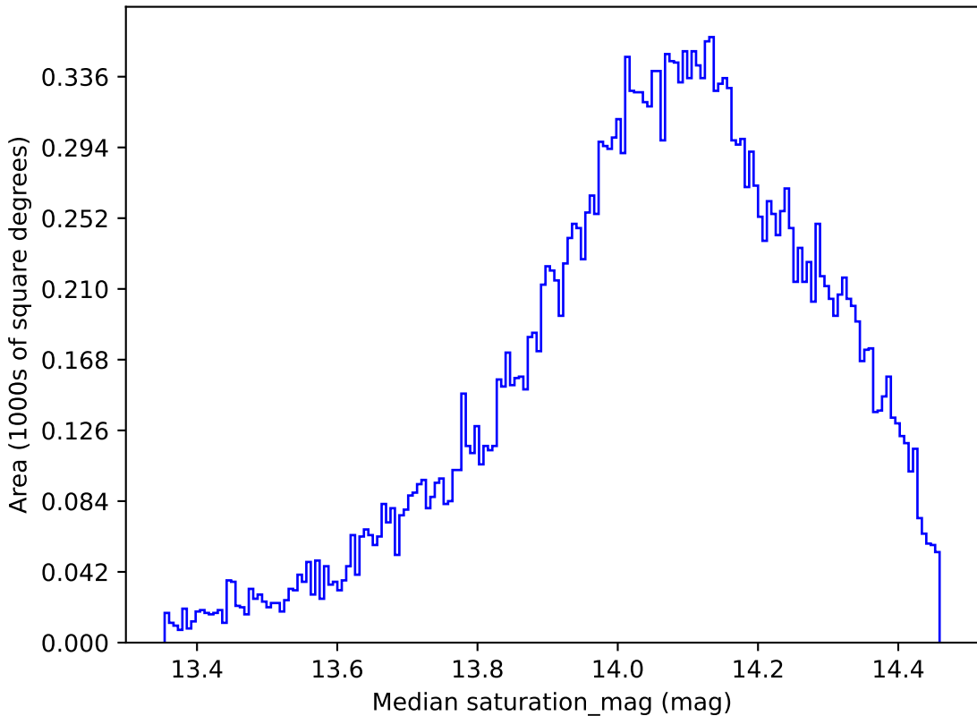
scp_reweight_v3.3_10yrs All sky z band: Median saturation_mag
