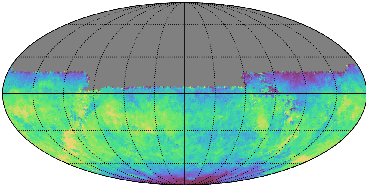
scp_reweight_v3.3_10yrs All sky u band: Median saturation_mag
