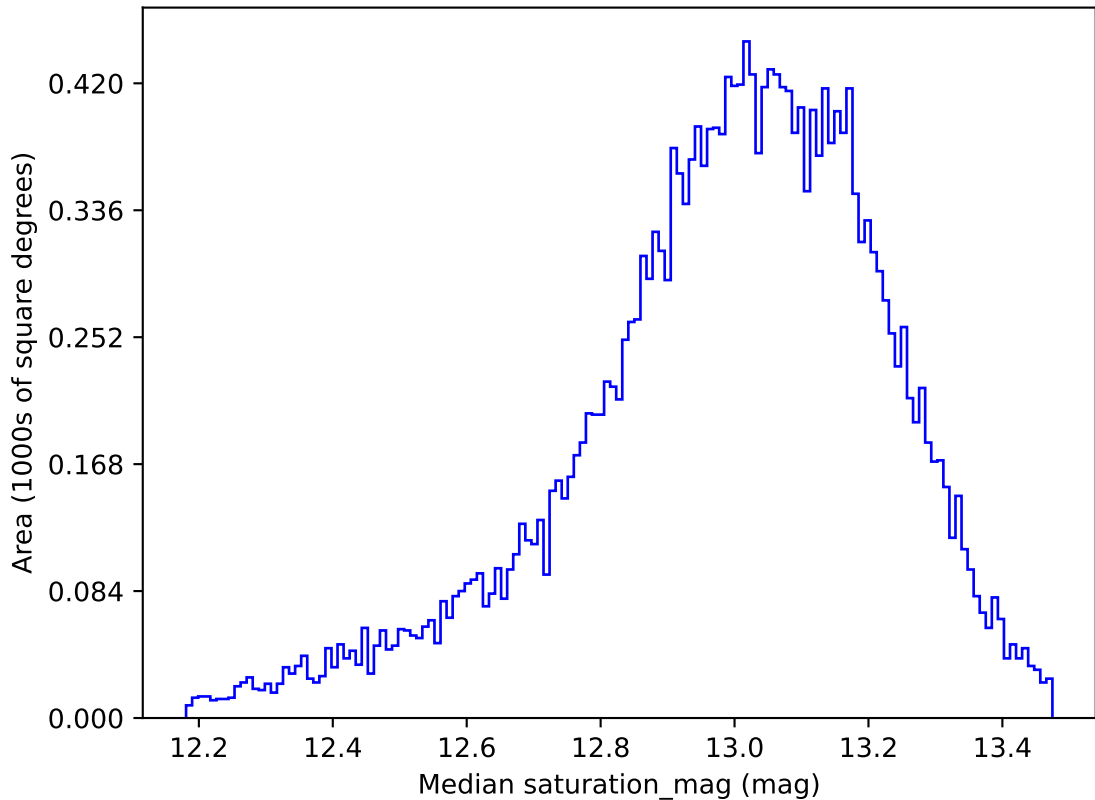
scp_reweight_v3.3_10yrs All sky u band: Median saturation_mag
