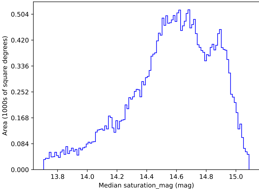
scp_reweight_v3.3_10yrs All sky r band: Median saturation_mag
