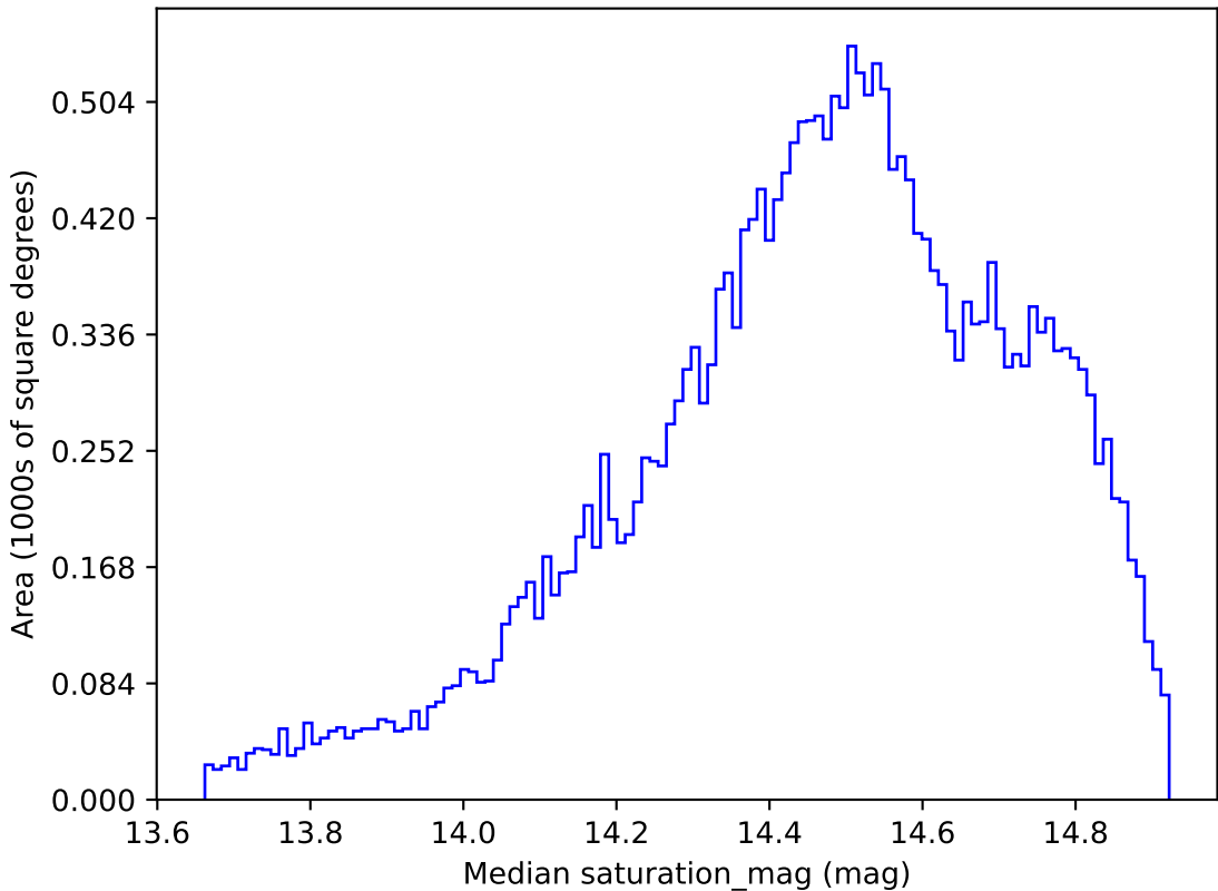
scp_reweight_v3.3_10yrs All sky i band: Median saturation_mag
