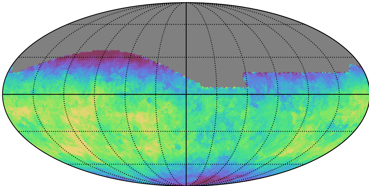
scp_reweight_v3.3_10yrs All sky g band: Median saturation_mag
