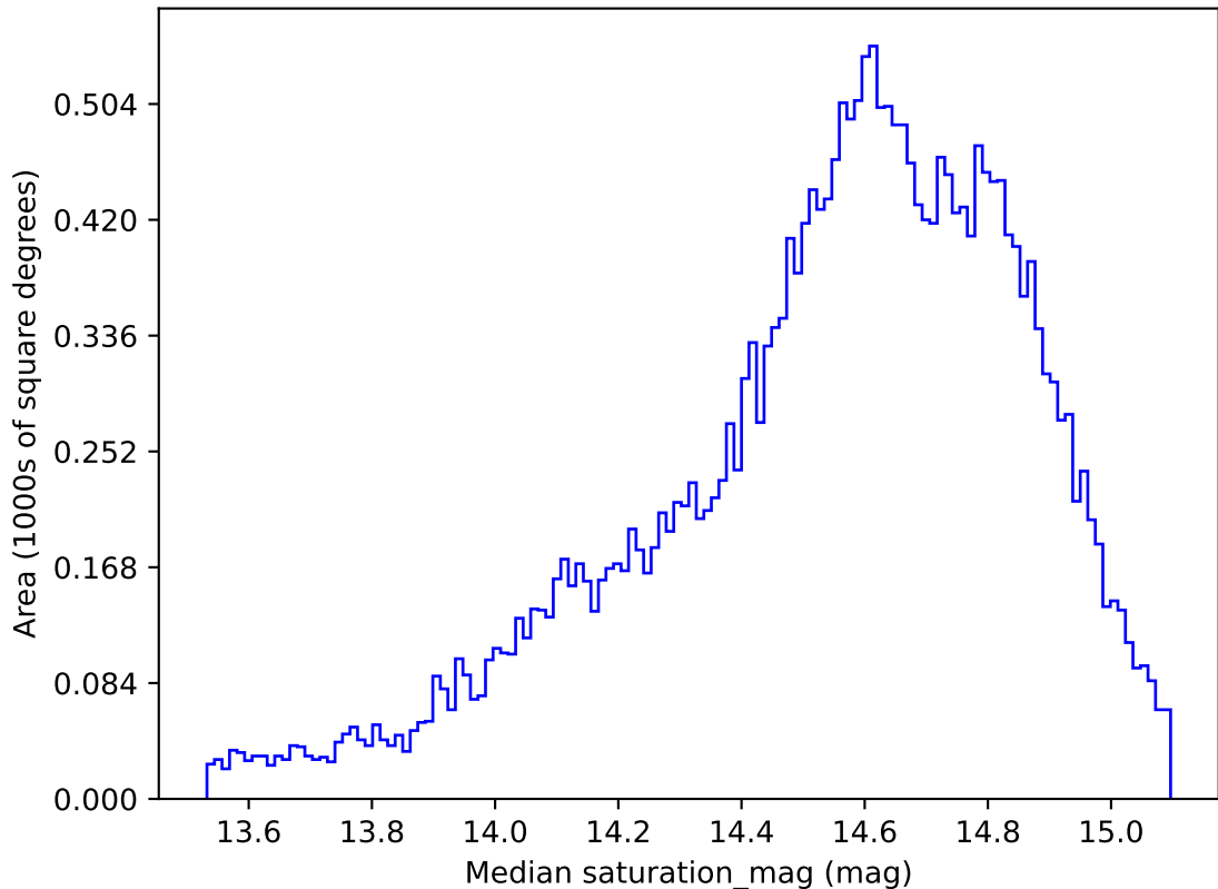
scp_reweight_v3.3_10yrs All sky g band: Median saturation_mag
