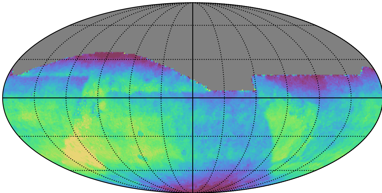
scp_reweight_v3.3_10yrs All sky all bands: Median saturation_mag
