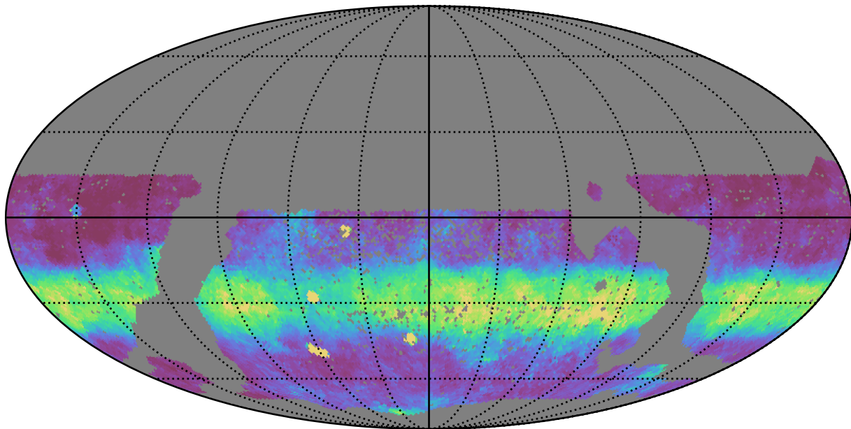
scp_reweight_v3.3_10yrs WFD z band: Median normairmass
