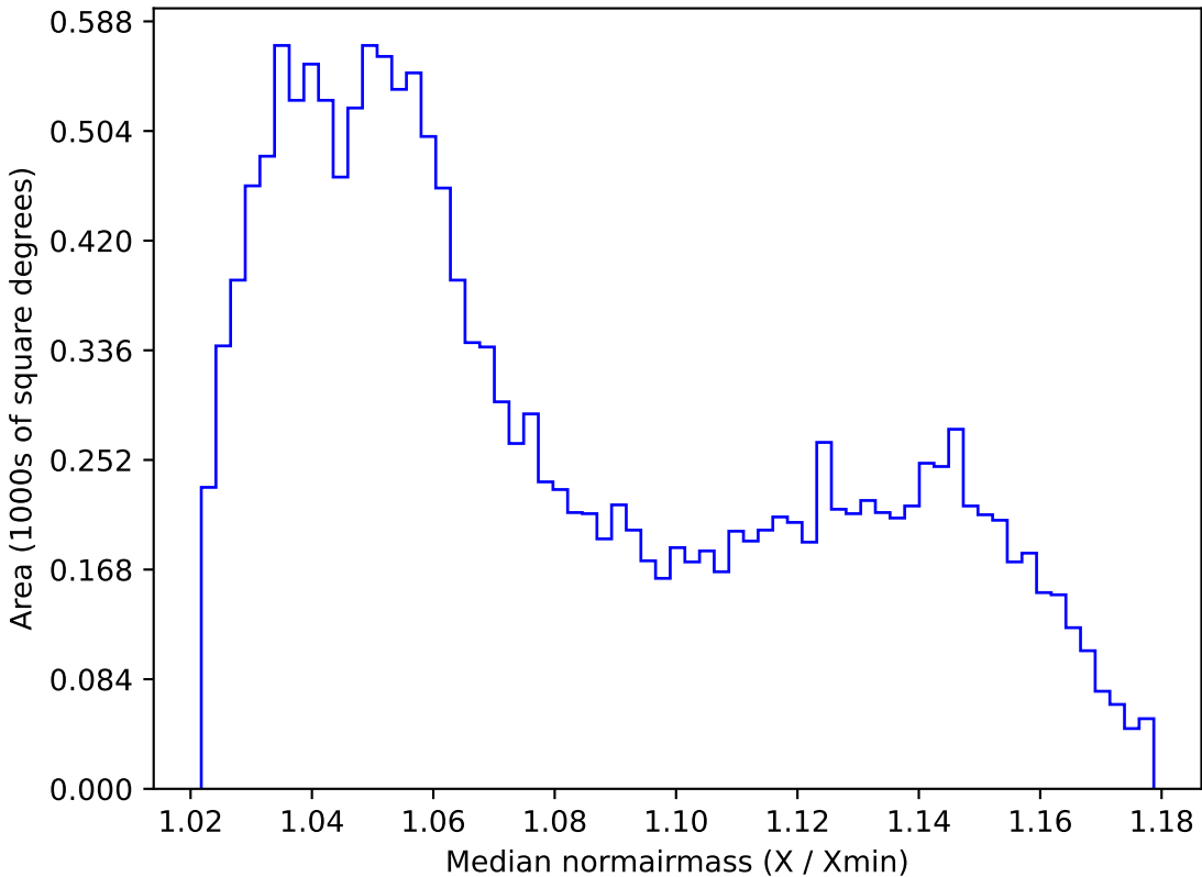
scp_reweight_v3.3_10yrs WFD z band: Median normairmass
