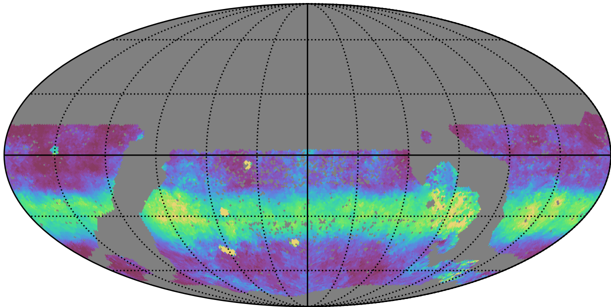
scp_reweight_v3.3_10yrs WFD y band: Median normairmass
