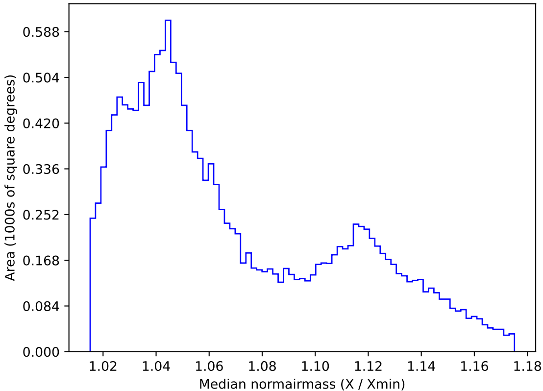
scp_reweight_v3.3_10yrs WFD r band: Median normairmass
