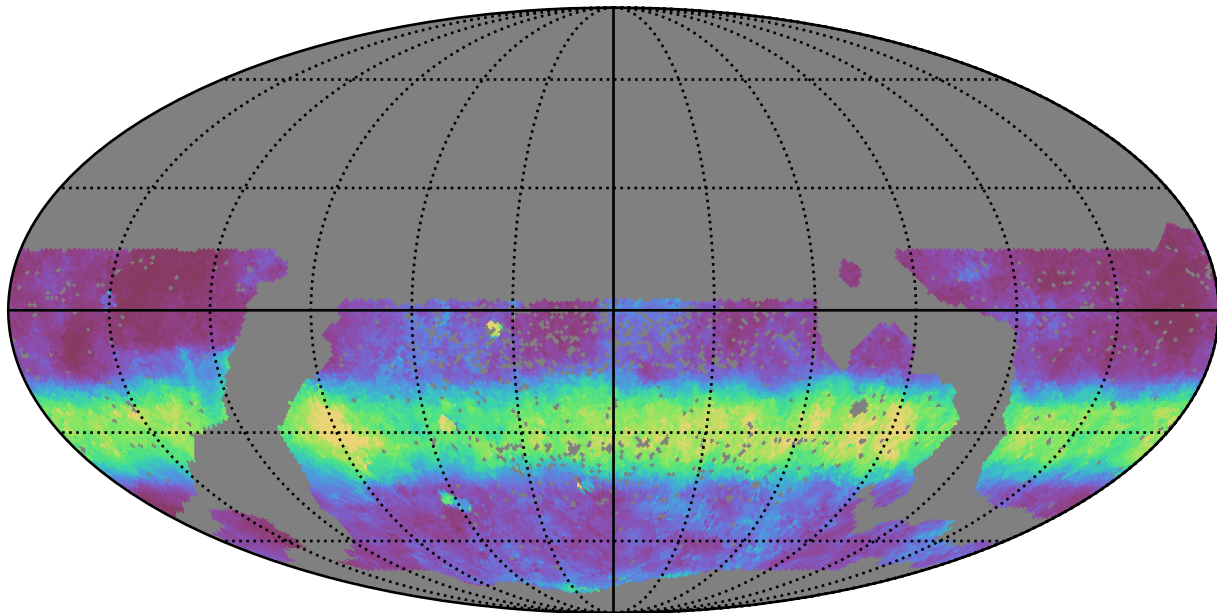
scp_reweight_v3.3_10yrs WFD i band: Median normairmass
