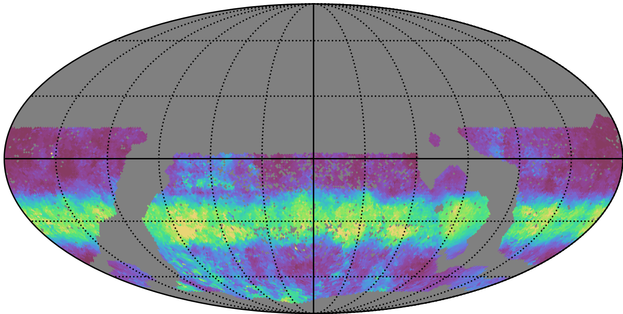
scp_reweight_v3.3_10yrs WFD g band: Median normairmass
