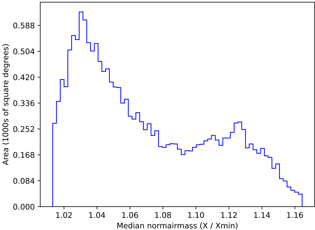
scp_reweight_v3.3_10yrs WFD g band: Median normairmass
