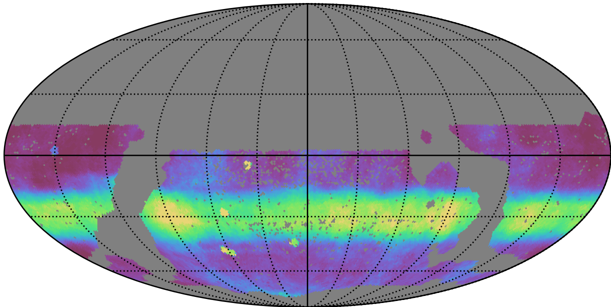
scp_reweight_v3.3_10yrs WFD all bands: Median normairmass
