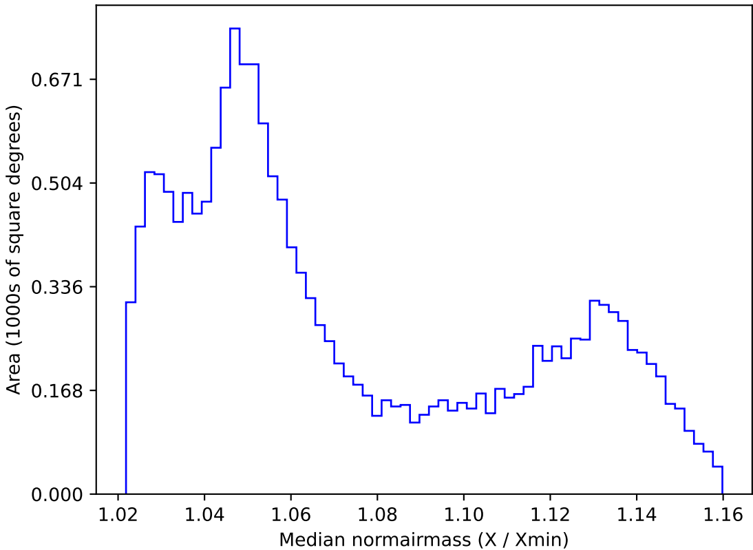
scp_reweight_v3.3_10yrs WFD all bands: Median normairmass
