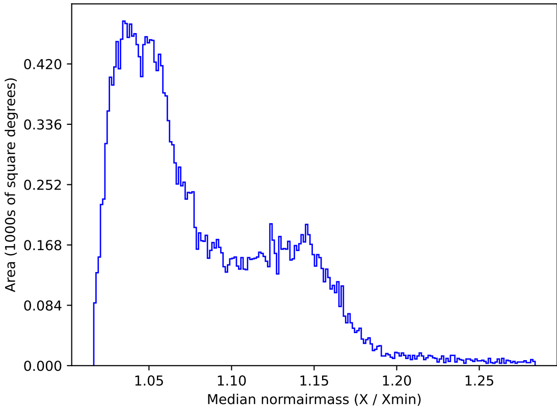
scp_reweight_v3.3_10yrs All sky z band: Median normairmass
