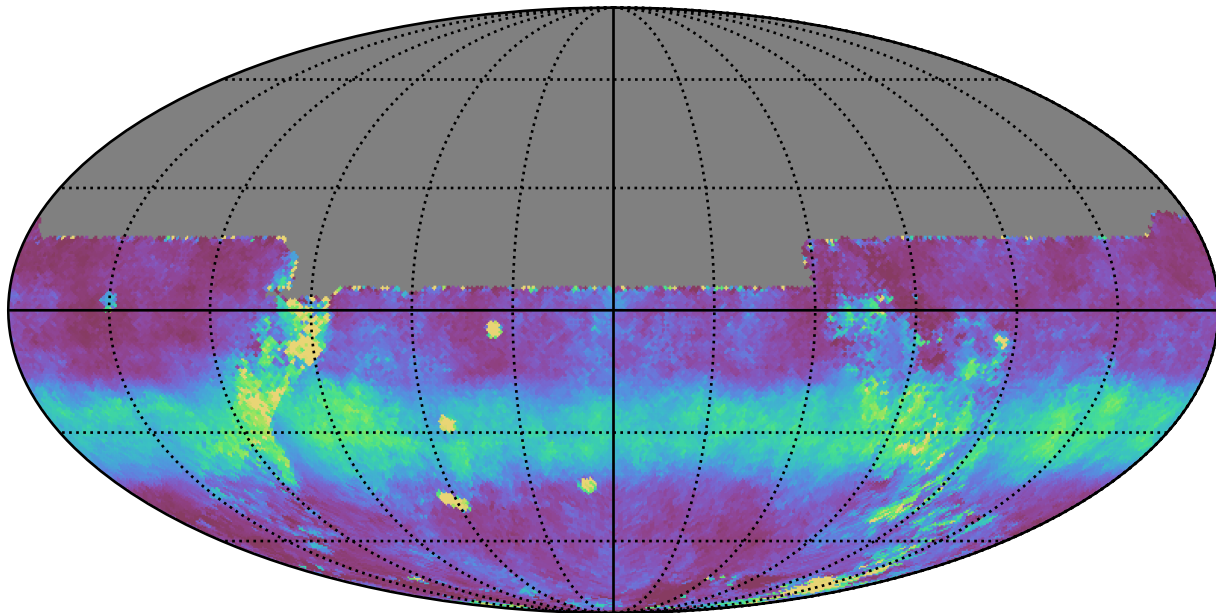
scp_reweight_v3.3_10yrs All sky y band: Median normairmass
