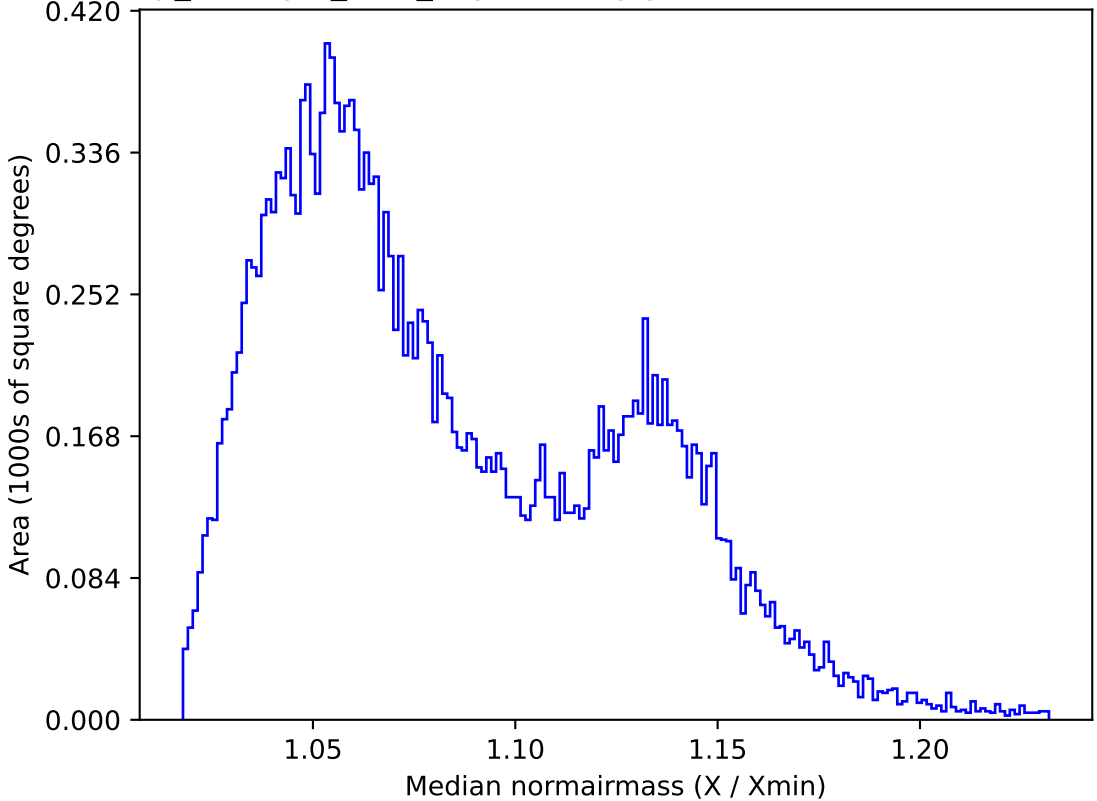
scp_reweight_v3.3_10yrs All sky y band: Median normairmass
