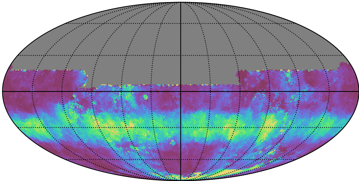
scp_reweight_v3.3_10yrs All sky u band: Median normairmass
