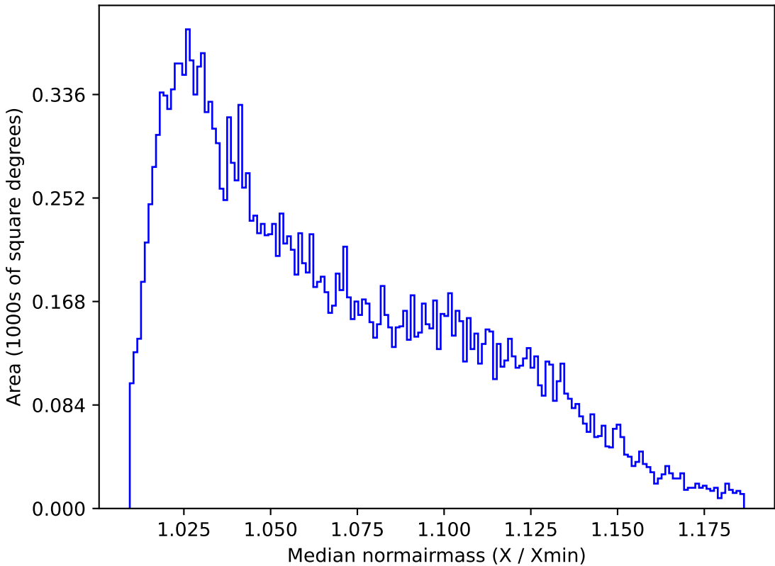
scp_reweight_v3.3_10yrs All sky u band: Median normairmass
