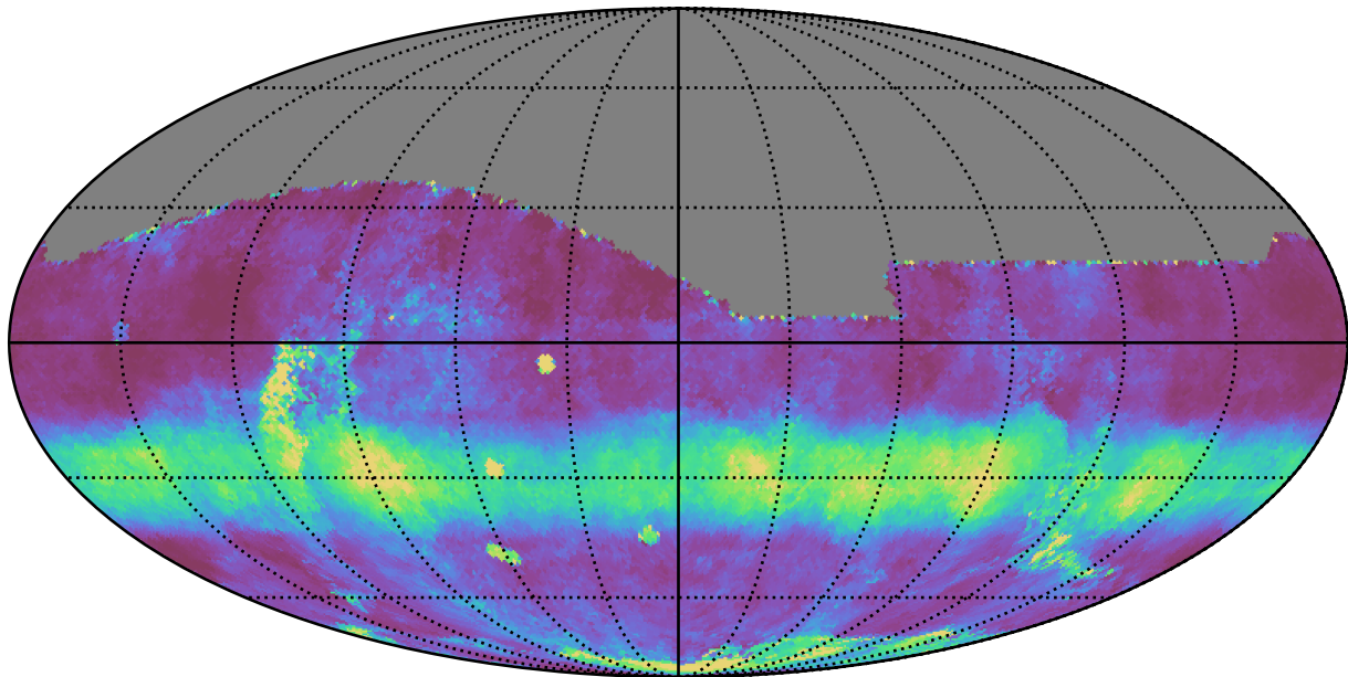
scp_reweight_v3.3_10yrs All sky r band: Median normairmass
